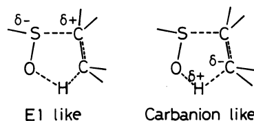
Fig. 3. E1-like and Carbonion-like cyclic transition states.
